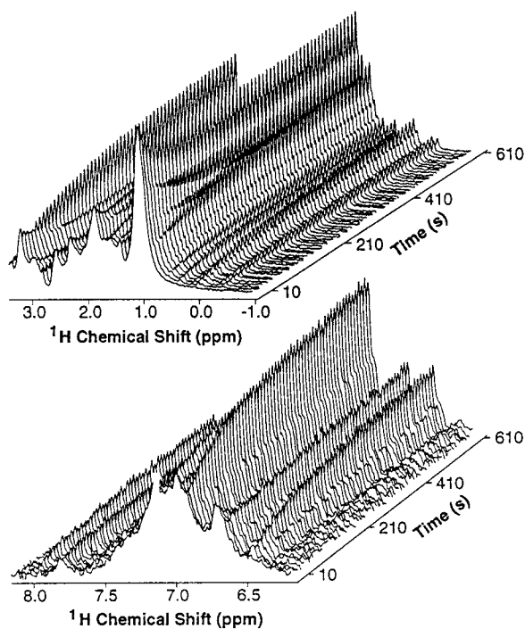
FIGURE 2. Stack plot of 1-D NMR spectra of BLA. 42 For the refolding experiment, BLA in 6 M GdnDCI (d, Figure 1) was diluted into a refolding buffer containing EDTA (to sequester the \text{Ca}^{2+} ions; e, Figure 1), and ^1\text{H} NMR spectra were recorded at 20 °C at incremented time points (between 1.2 s and 10.3 min) after initiation of refolding. The region shown at the top contains resonances from methyl and methylene groups, and that at the bottom from aromatic residues.
